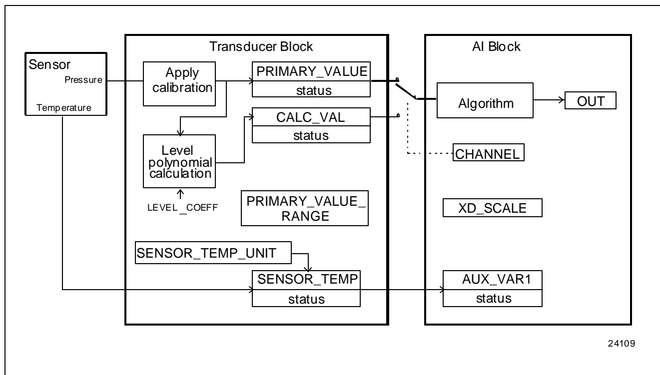
Figure 4 ¾ Transducer and Analog Input Function Block Diagram
