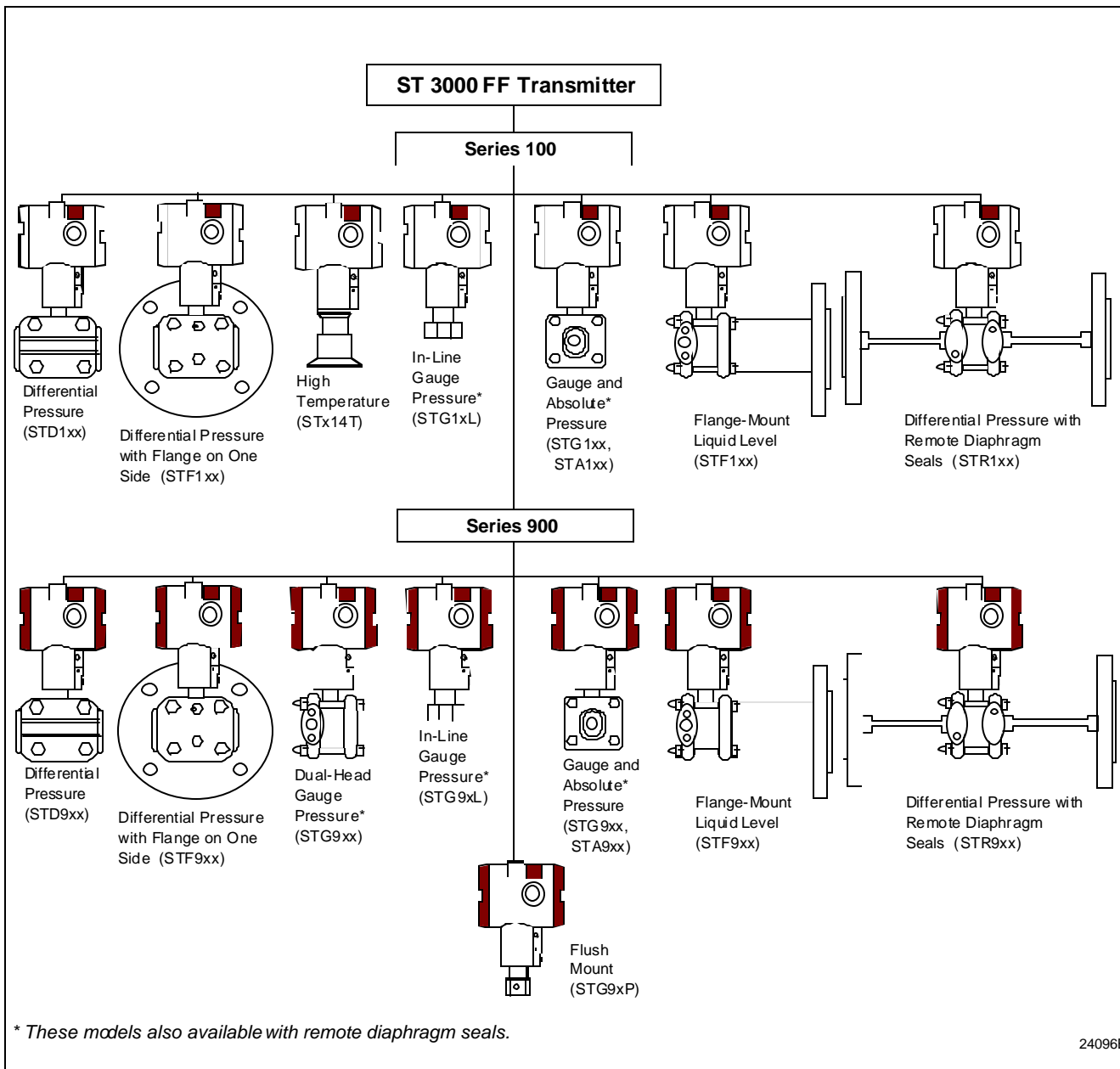
Figure 2 ¾ ST 3000 Fieldbus Transmitter Family Tree
